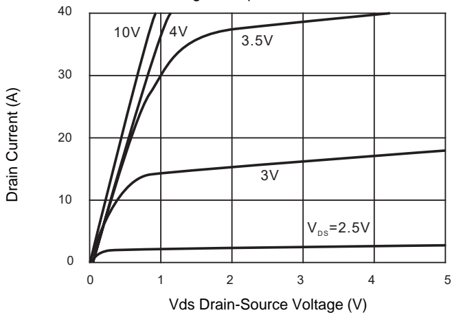
Fig. 1-Output Characteristics
