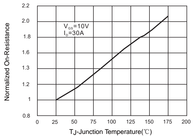
Fig. 2-Rdson-JunctionTemperature
